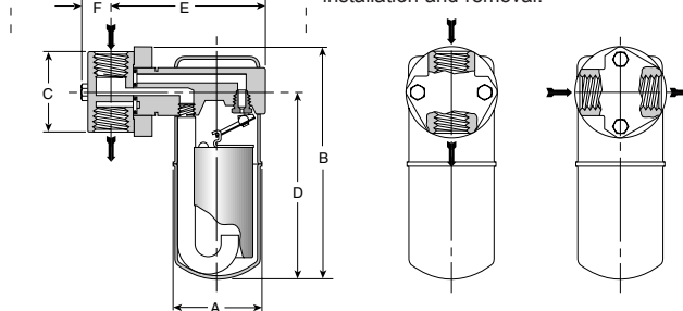
Model 2011 Trap With Standard Connector
